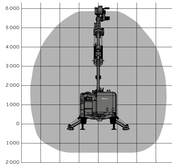
Horizontal drilling forwards with hydraulic rollover
