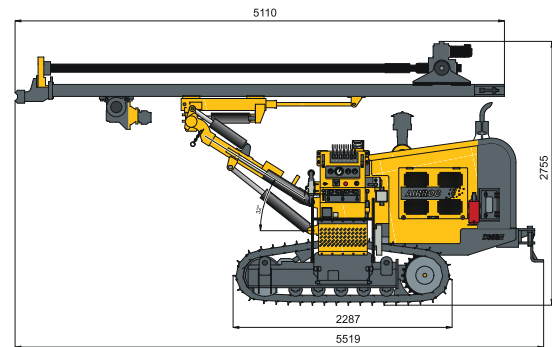
Transport dimension
